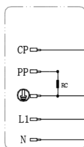
Vehicle Connector wiring diagram
